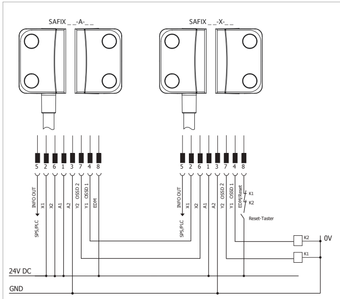
Figure 10: Direct connection of two protections according to PL e, SAFIX __-A-__ & SAFIX __-X-__
